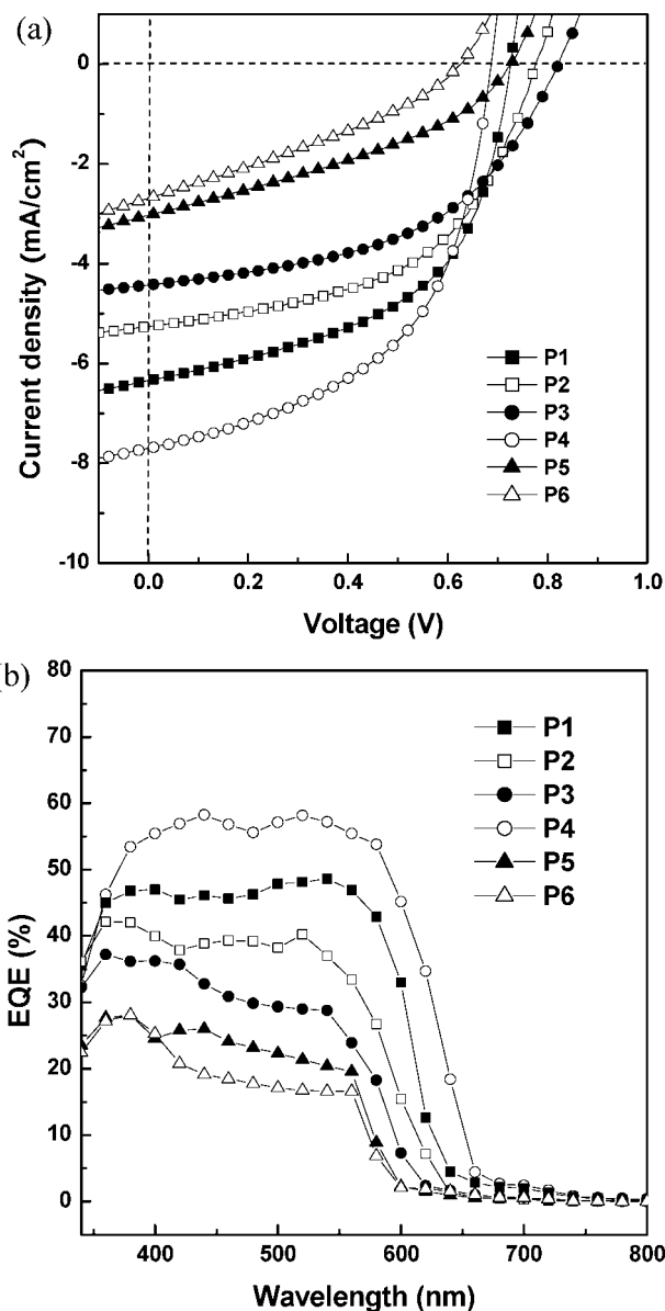
Figure 4. (a) I - V curves (under simulated AM 1.5 solar irradiation) and (b) EQE wavelength dependencies of PSC devices with an active layer of blended copolymers P1–P6 :PCBM (1:1 w/w).
